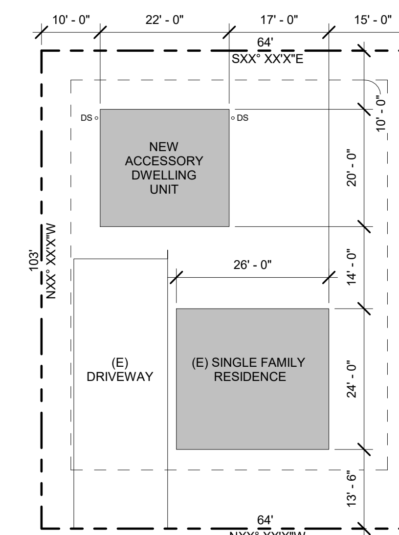
1 EXAMPLE SITE PLAN SCALE: 1/16" = 1'-0"
