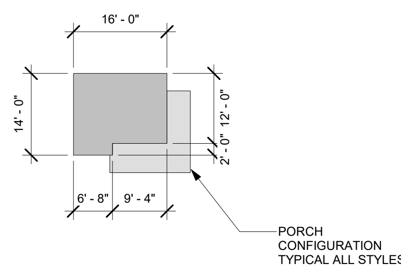
5 PLAN 1 - ALL PLANS SCALE: 1/16" = 1'-0"
