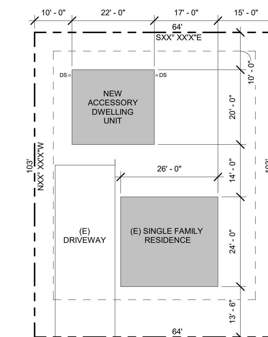
1 EXAMPLE SITE PLAN A1-201 | AS-106 | SCALE: 1/16" = 1'-0"
