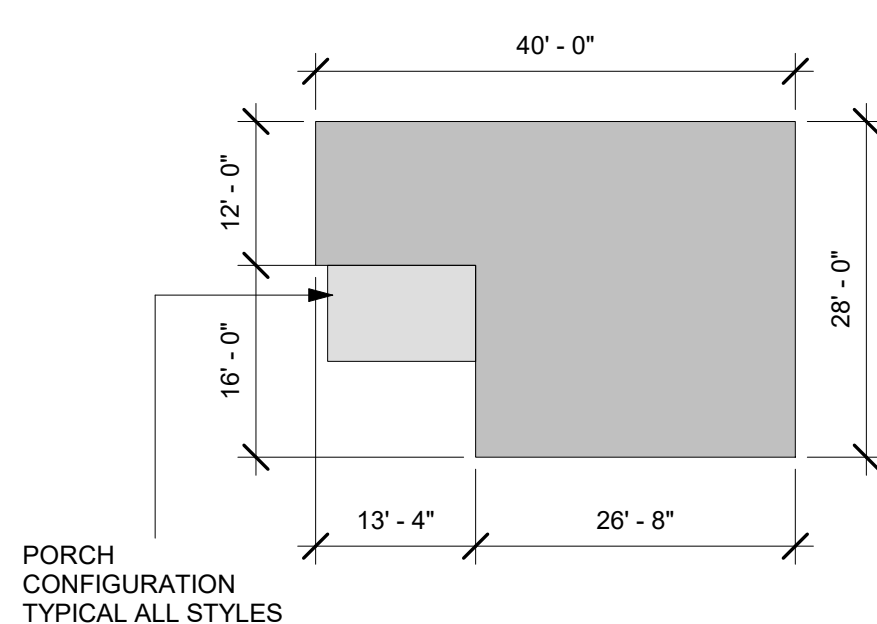
5 PLAN 6 - ALL STYLES A1-201 | AS-106 | SCALE: 1/16" = 1'-0"
